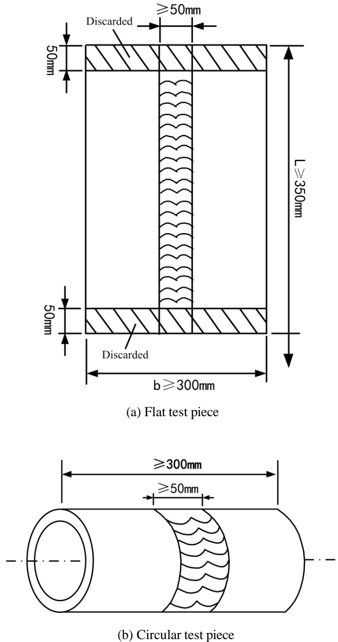
Figure 4.4.3-(1) Specimen size for additive repair process approval test
