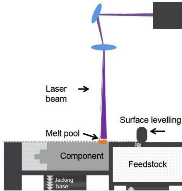
Figure 2.3.2 Powder bed fusion process
