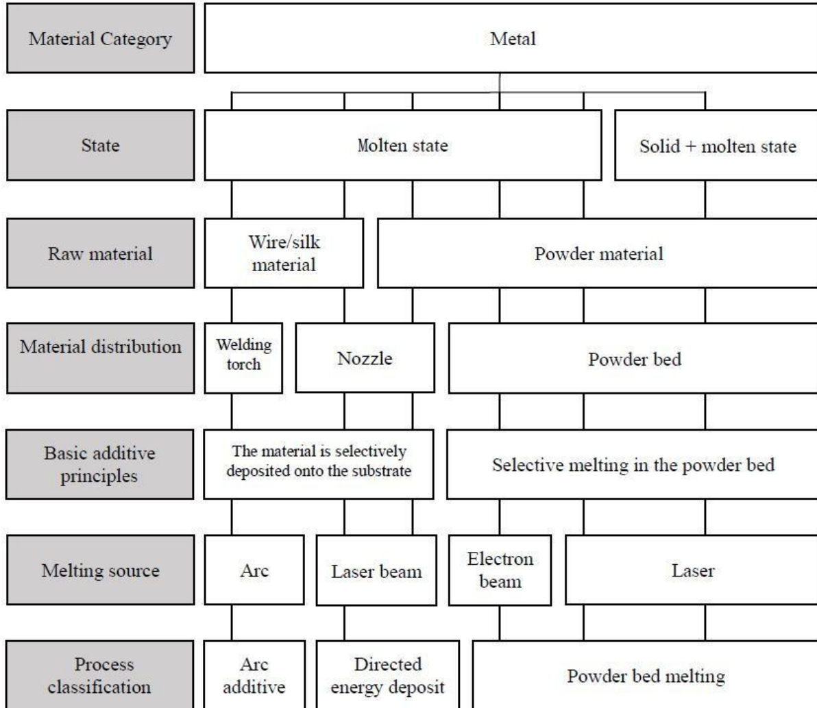
Figure 4.3.2.3 Metal material additive manufacturing process flow chart
