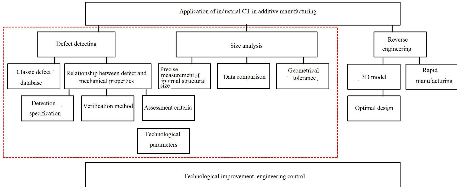
Figure B.1 Flowchart of Application of Industrial CT detection in Additive Manufacturing
