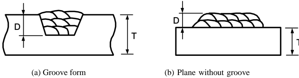
Figure 4.3.3-(2) Edge preparation of specimen
